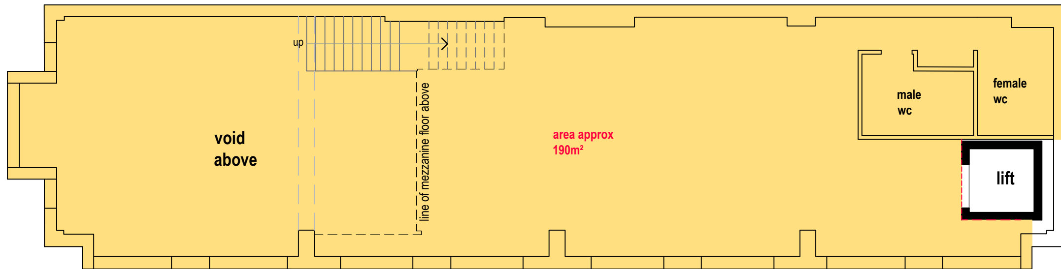
L1 FLOOR PLAN
